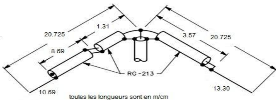
Antenne 80m large bande
